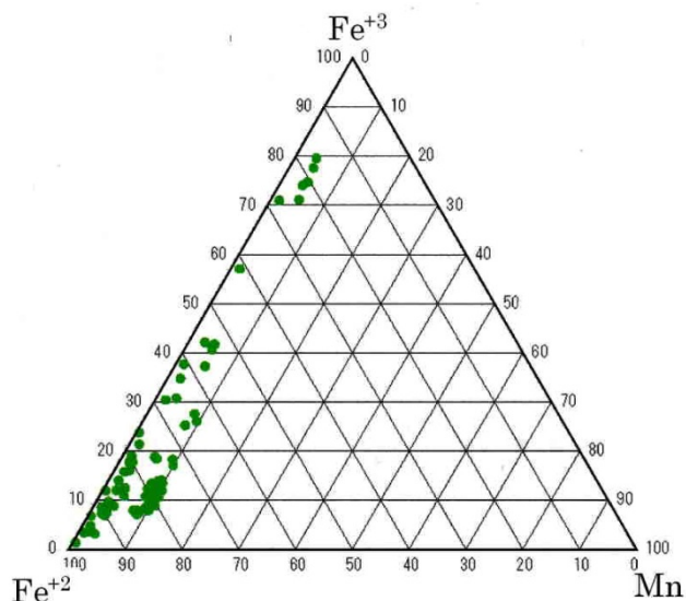
Fig. 14 \text{Fe}^{+3}:\text{Fe}^{+2}:\text{Mn} atomic ratio (%) for ilmenite in diorite.
