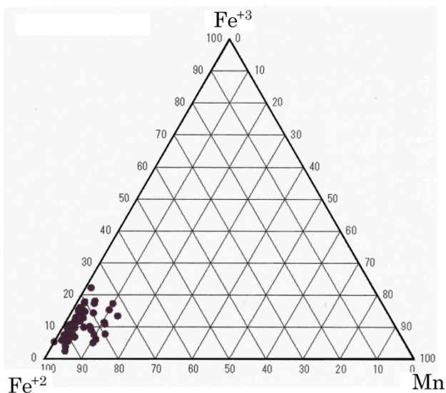
Fig. 15 \text{Fe}^{+3}:\text{Fe}^{+2}:\text{Mn} atomic ratio (%) for ilmenite in two-pyroxene gabbro.
