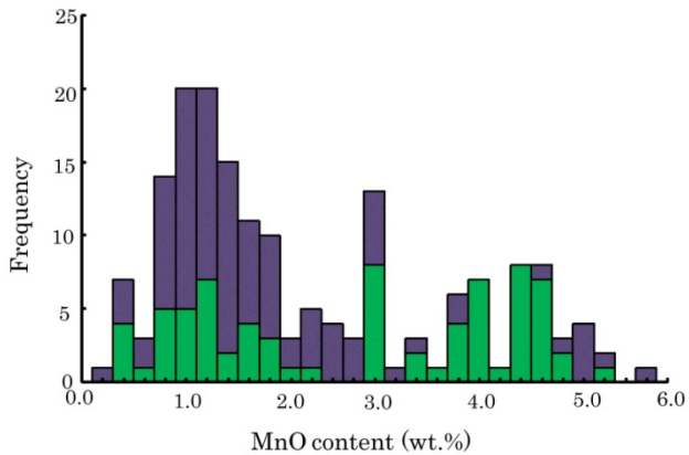
Fig. 13. Histogram of vanadium content as MnO in ilmenite from the Kouyama gabbroic body.
