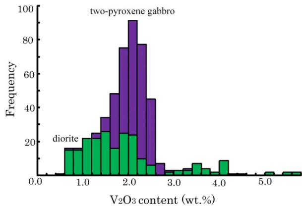
Fig. 10. Histogram of vanadium content as V_2O_3 in magnetite from the Kouyama gabbroic body.
