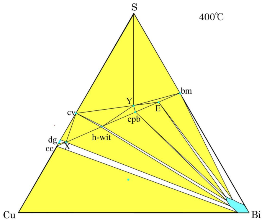
Figure 3-2-4. Isothermal section of Cu-Bi-S system at 400°C. (compiled after Nomiyama 1968) 12) .
