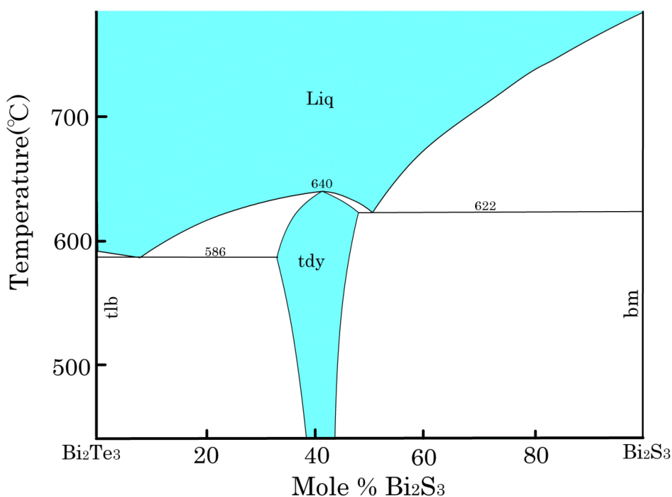
Fig. 3-1-1. Phase diagram for \text{Bi}_2\text{Te}_3 - \text{Bi}_2\text{S}_3 join in the Bi-Te-S system above 450°C (modified after Yusa; 1979 7) ).
