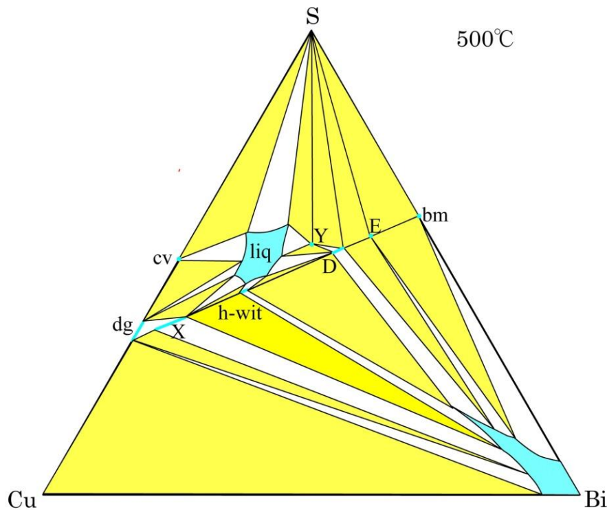
Figure 3-2-2. Isothermal section of Cu-Bi-S system at 500°C (compiled after Nomiyama 1968) 12) .
