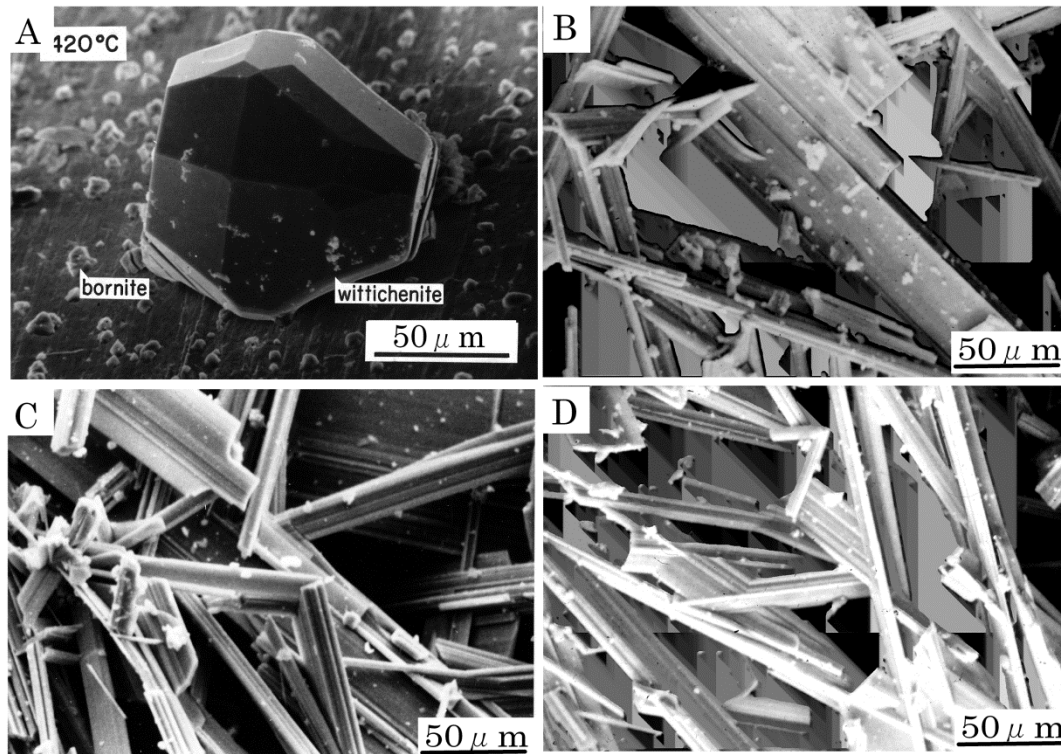
Figure 3-2-9. Hydrothermally synthetic minerals of SEM photographs.
