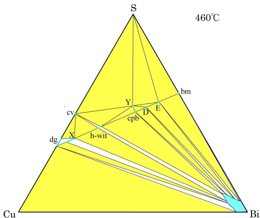
Figure 3-2-3. Isothermal section of Cu-Bi-S system at 460°C (compiled after Sugaki et al. , 1980) 11) .
